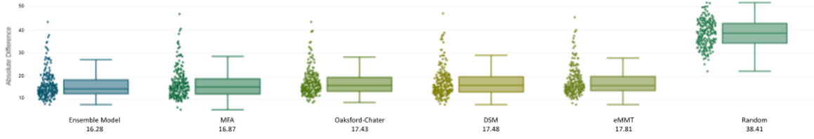
Figure 2: Boxplot depicting individual performance through the absolute difference between the predicted value and the true response. Overall mean absolute difference beneath the model’s name. The comparable performance between OC, DSM and \epsilon -MMT points to (a partial) functional equivalence.
